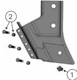
688-HLD-5000 FITS: Horsch 84° Shank NOTES: On older drills, customer needs to verify mounting bolt holes. 1/2" bolt hole requires 694-HLD-5000 (does not require 694-ACC-1000) 5/8" bolt hole requires 688-HLD-5000
